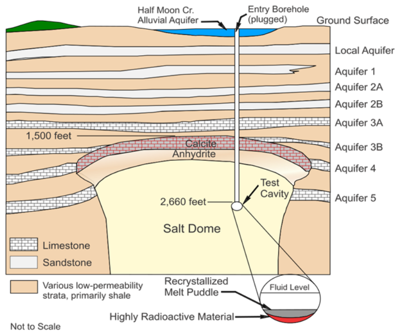
Figure 14. Test Cavity and Aquifers at the Salmon Test Site
