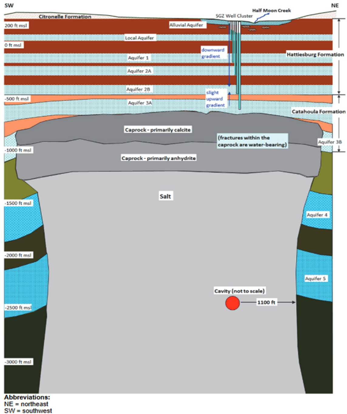
Figure 25. Conceptual Model of the Relationship of the Dome, Shot Cavity, and SGZ Well Cluster at the Salmon Site
