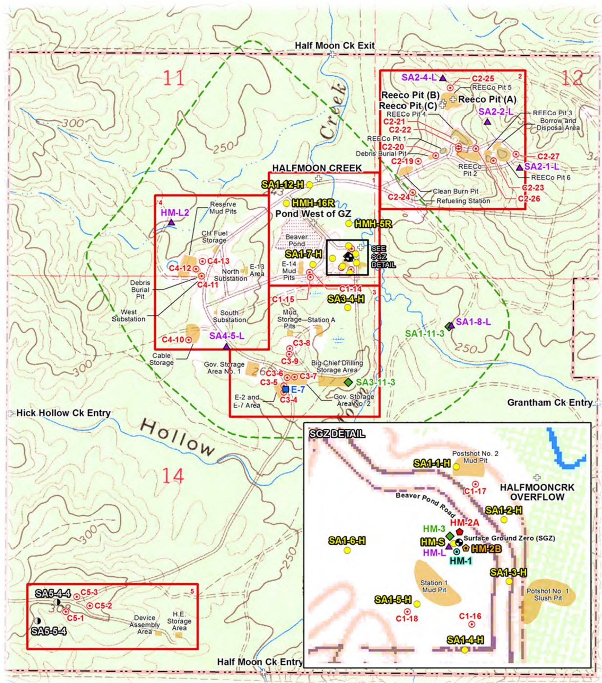
Figure 15. SGZ Downhole Wells and Other Onsite Sample Locations
