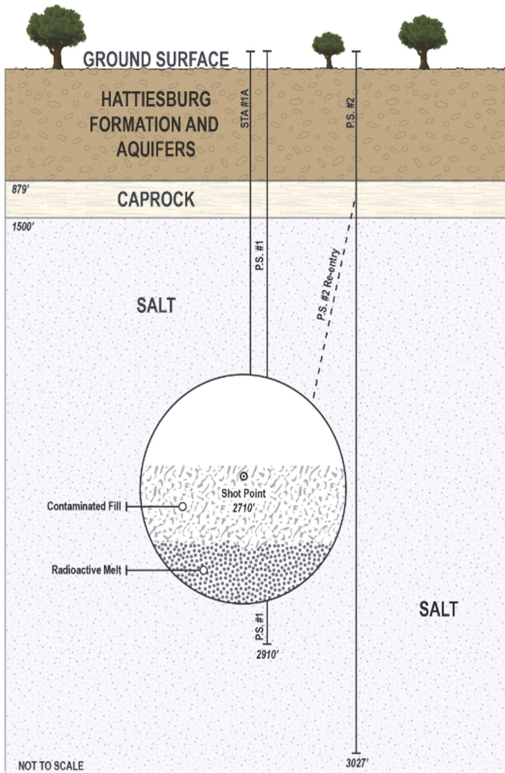
Figure 24. Cross-sectional Depiction of the shot Cavity After Surface Decommissioning
