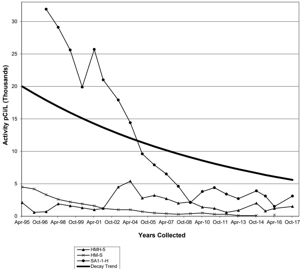
Figure 17. Tritium Trend Chart for Selected Sample Points
