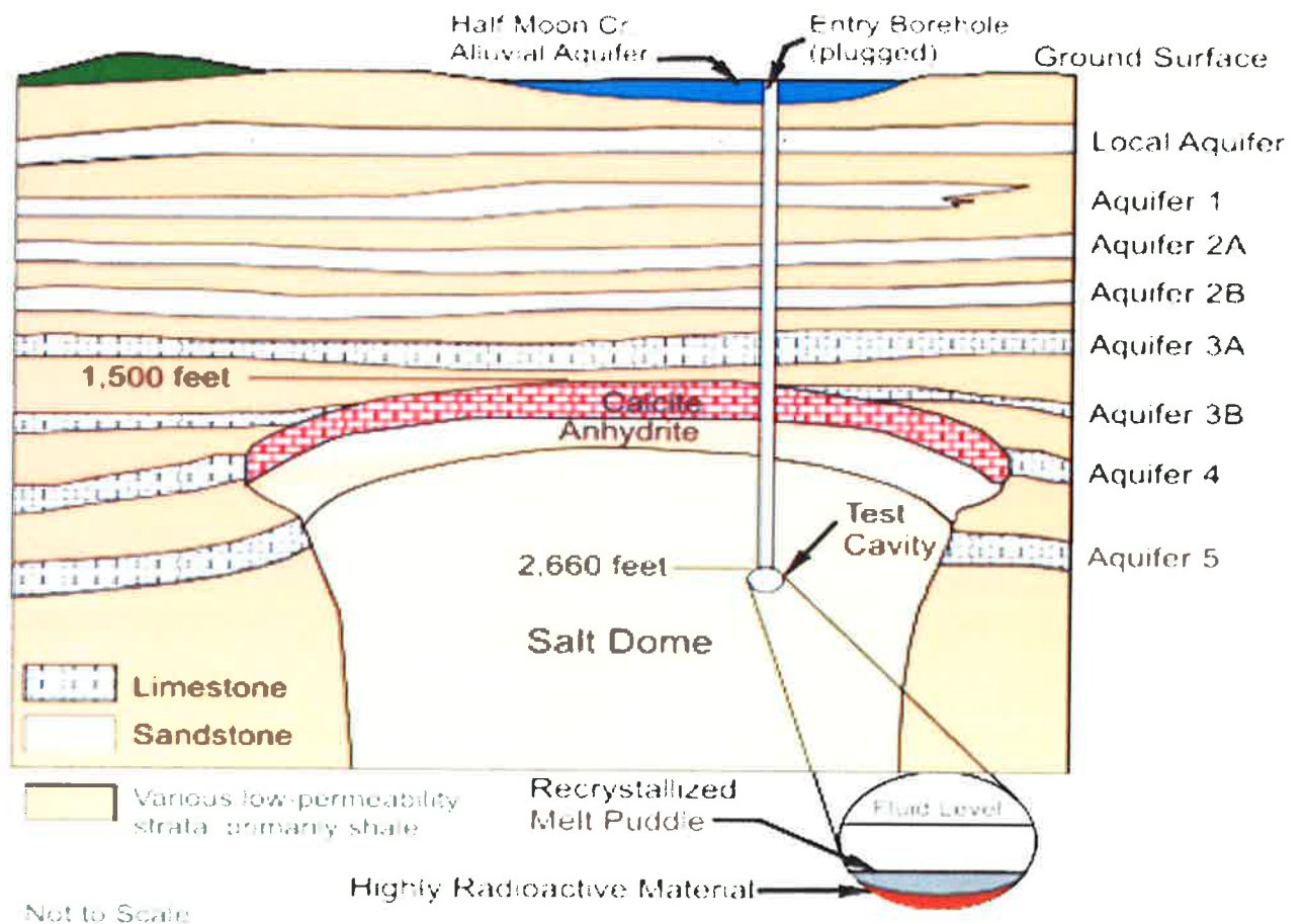
Figure 2, Test Cavity and Aquifers at the Salmon Test Site
